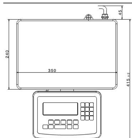
Front-mounted display
