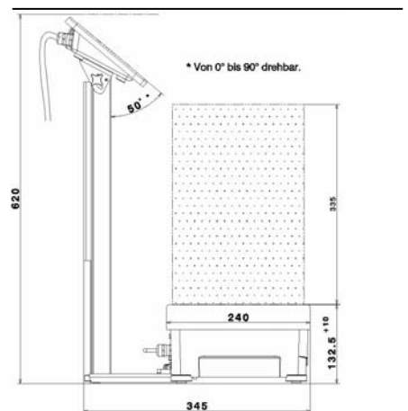
Raised display with YDH01P column
